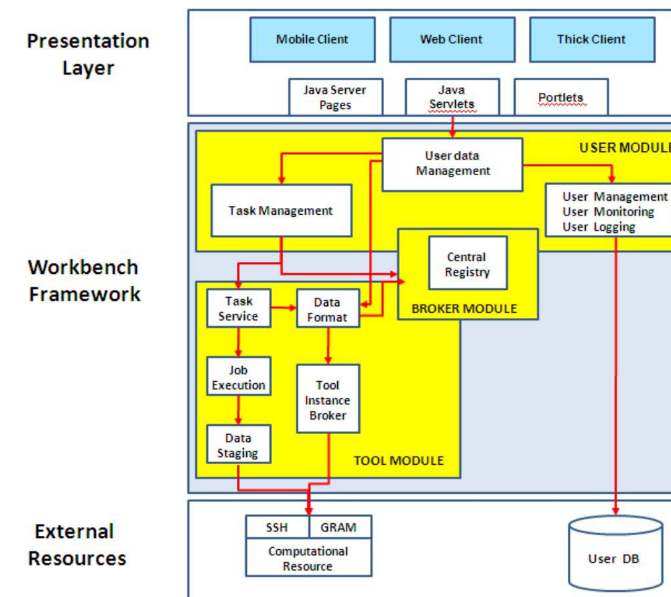
Figure 3. The NSG's architecture uses WF, which contains modules to manage submission of jobs to analytical tools on computational resources, and modules to manage queries on data resources. Presentation Layer: Supports access by browser clients and programmatic access via SOAP [SOAP] and ReST [Fielding 2000] services. User Module: Manages all user-initiated activities, passing queries and tasks to executive portions of the infrastructure; stores user and task information; manages user roles, account assignments, data sharing between accounts, access to tools and data sources (which may be proprietary). Broker Module: Stores and provides access to application-specific information in a Central Registry, e.g. input and output data types for each application. Tool Module: Translates user-submitted tasks into command lines, submits commands and user data to appropriate compute engine for execution. External Resources: Can be accessed via SSH, GRAM/Globus [GLOBUS], SOAP, ReST etc..
